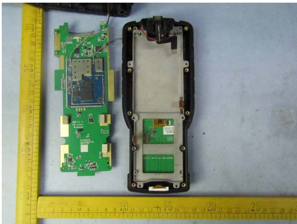
Fig. 6 -- Inside view
