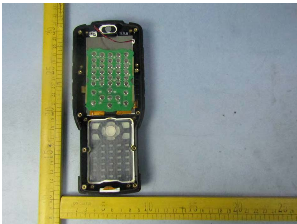
Fig. 8 -- PCB view 1
